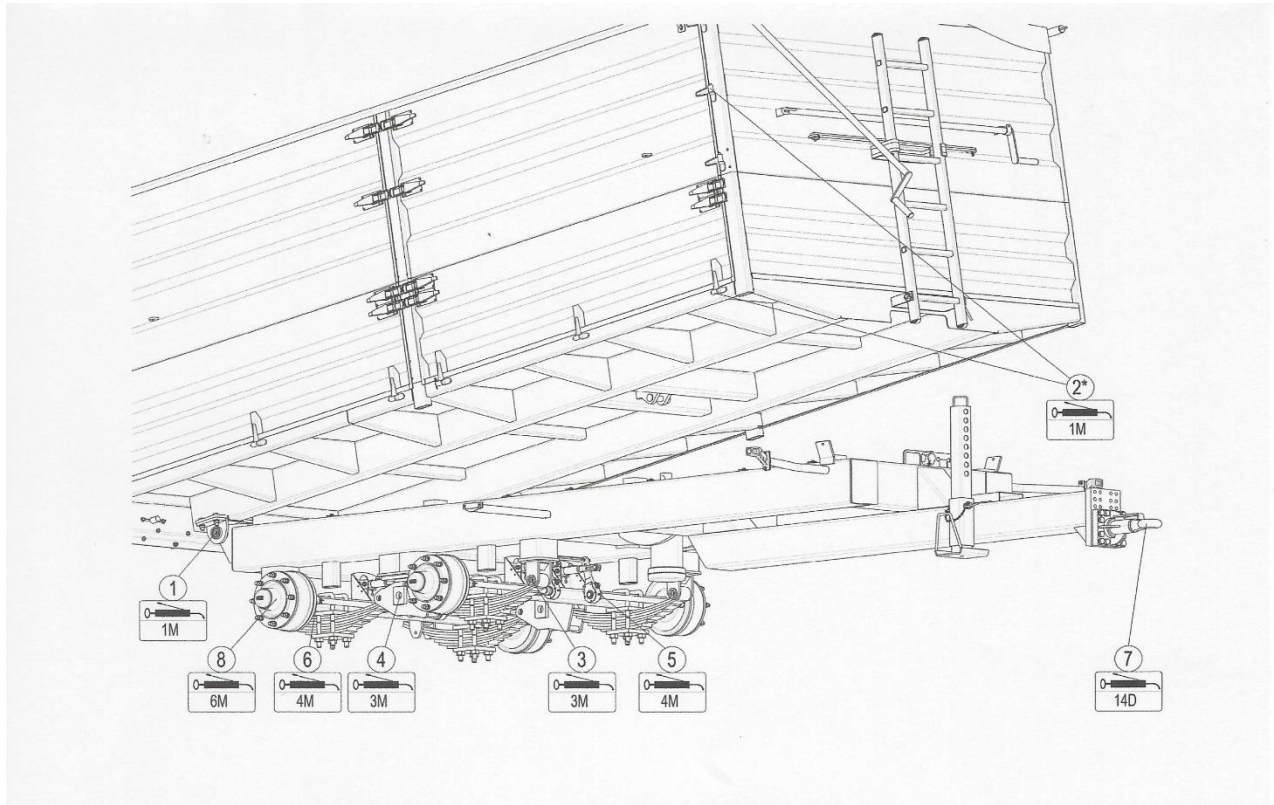
Fig. 11 Greasing places
