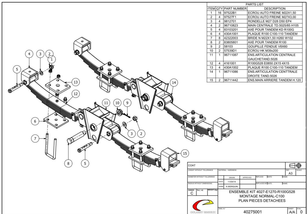
Figure 9: GD4-14 Suspension Parts List
