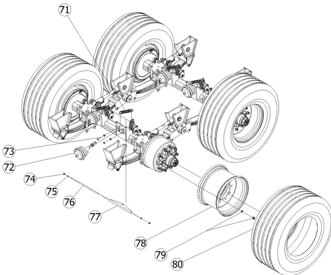
Figure 4: Brake Parts
