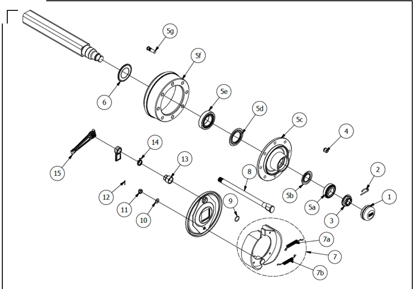
Figure 3 GD100;GD125;GD140 Axle
