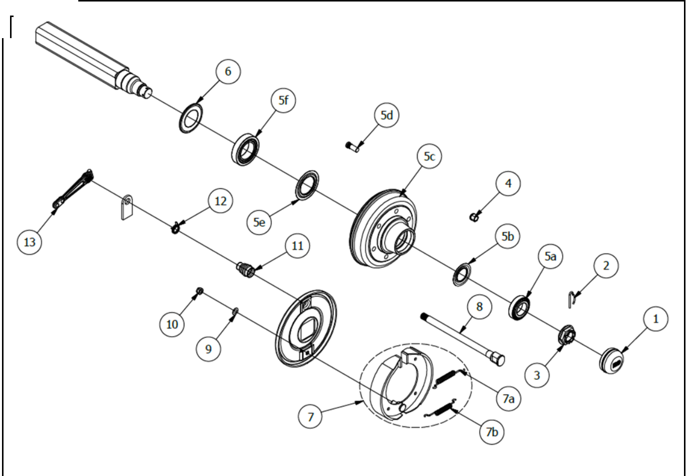
Figure 4 GD85 Axle
